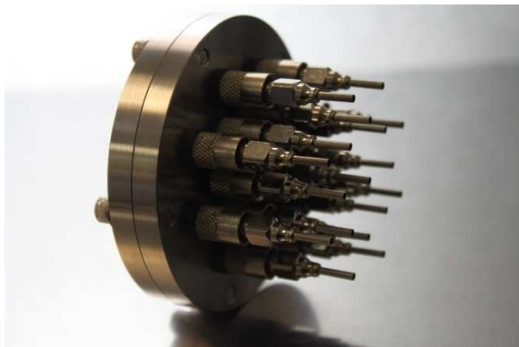
Side view with all (17) output needles installed
